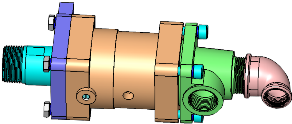
Three-dimensional Drawing of WDSG32-15 Rotary Joint
