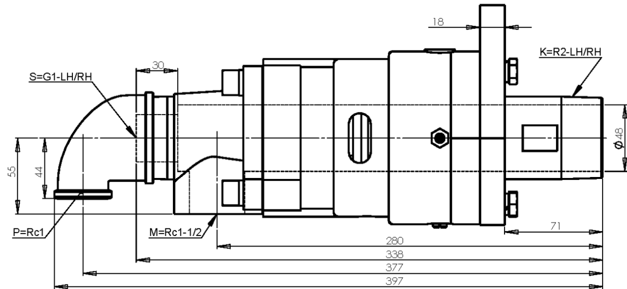
Surface Contour for Dual Flow WDSG50-25 Rotary Joint With Stationary Internal Pipe
