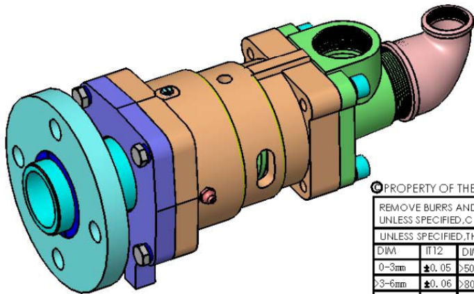
Surface Contour for Dual Flow WDS-GF50-25 Rotary Joint With Stationary Internal Pipe
