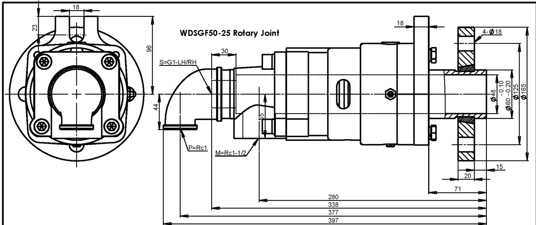
Surface Contour for Dual Flow WDS-GF50-25 Rotary Joint With Stationary Internal Pipe
